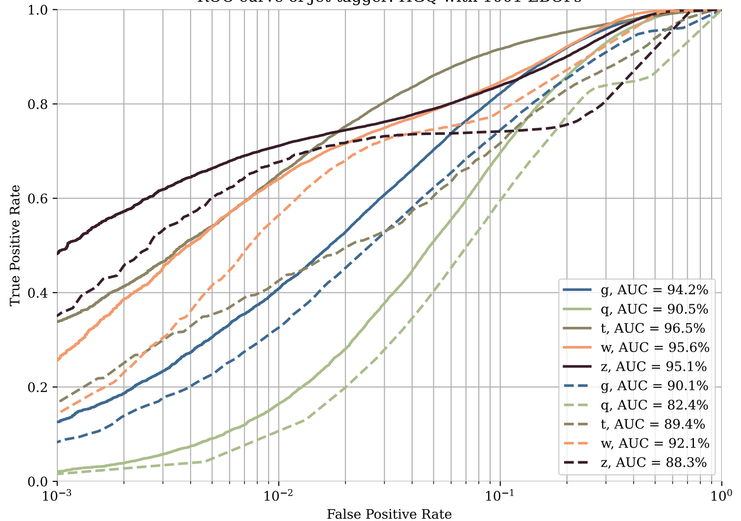
ROC-curve of Jet-tagger: HGQ with 1001 EBOPs
